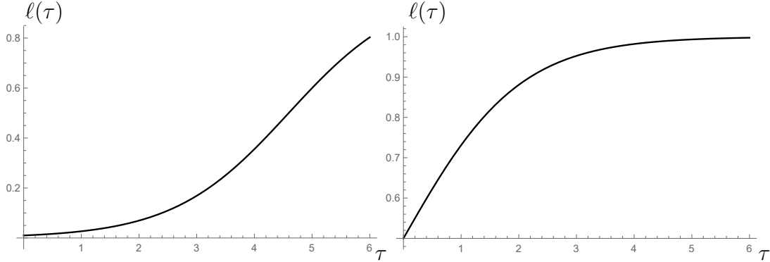
Figure 2: Function \ell(\tau) for a large group size on the left-hand side ( K = 100 ) and for a small group on the right-hand side ( K = 2 ); \gamma = 1 and the initial measure of infected is 1 in both graphs.
