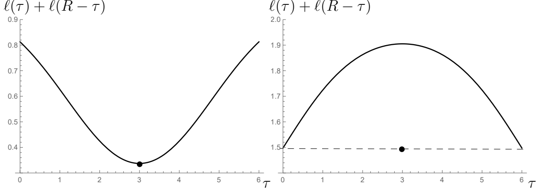
Figure 3: Function \ell(\tau) + \ell(R - \tau) for a large group size on the left-hand side ( K = 100 ) and for a small group on the right-hand side ( K = 2 ); \gamma = 1 and R = 6 in both graphs.
