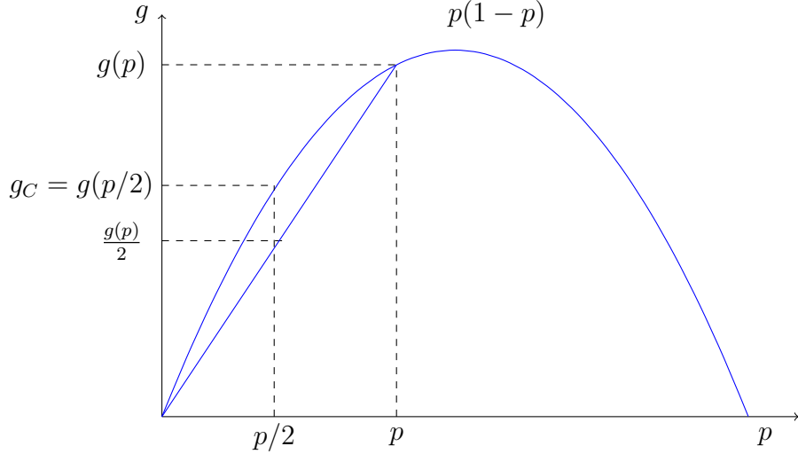
Figure 4: Mixing increases contagion.
