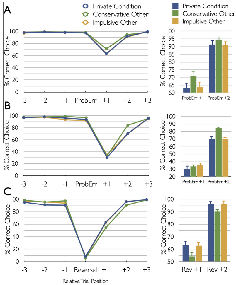
Fig. 3. Choice accuracy (for the truly correct color) as a function of trial position and social influence in Study 1. (A, B) Accuracy for trials –3 before to +3 after probabilistic errors (ProbErr, left) and in more detail for post-ProbErr trials +1 and +2 (right), split for first (A) and late (second/third, B) ProbErrs in a reversal episode. (C) Accuracy for trials –3 before to +3 after reversals (left) and in more detail for post-reversal trials +1 and +2 (right). Error bars show standard errors of the mean. (For interpretation of the references to colour in this figure legend, the reader is referred to the web version of this article.)
