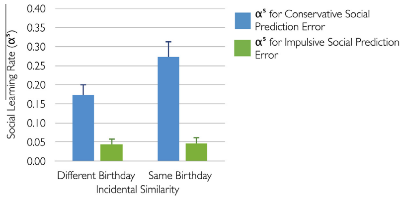
Fig. 5. Mean learning rates for \alpha^s derived from the best-fitting computational model and split for direction (conservative versus impulsive) of the \delta^s and the two groups of participants who observed another player either sharing (similar-other group) or not sharing (dissimilar-other group) their own birthday. Error bars show standard errors of the mean.
