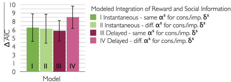
Fig. 4. Model fit comparisons in Study 1 using the Akaike Information Criterion (AIC), which corrects for the number of free parameters. The figure shows the differences \Delta AIC between the standard Q-learning model, which is based on \delta^s only ('social ignorer'), and the 4 integrative models in which both reward and social information are utilized, with the integration occurring either instantaneously or with a delay, and with applying either the same or different learning rates to conservative/impulsive \delta^s . A larger \Delta AIC indicates superior performance. Error bars show standard errors of the difference.
