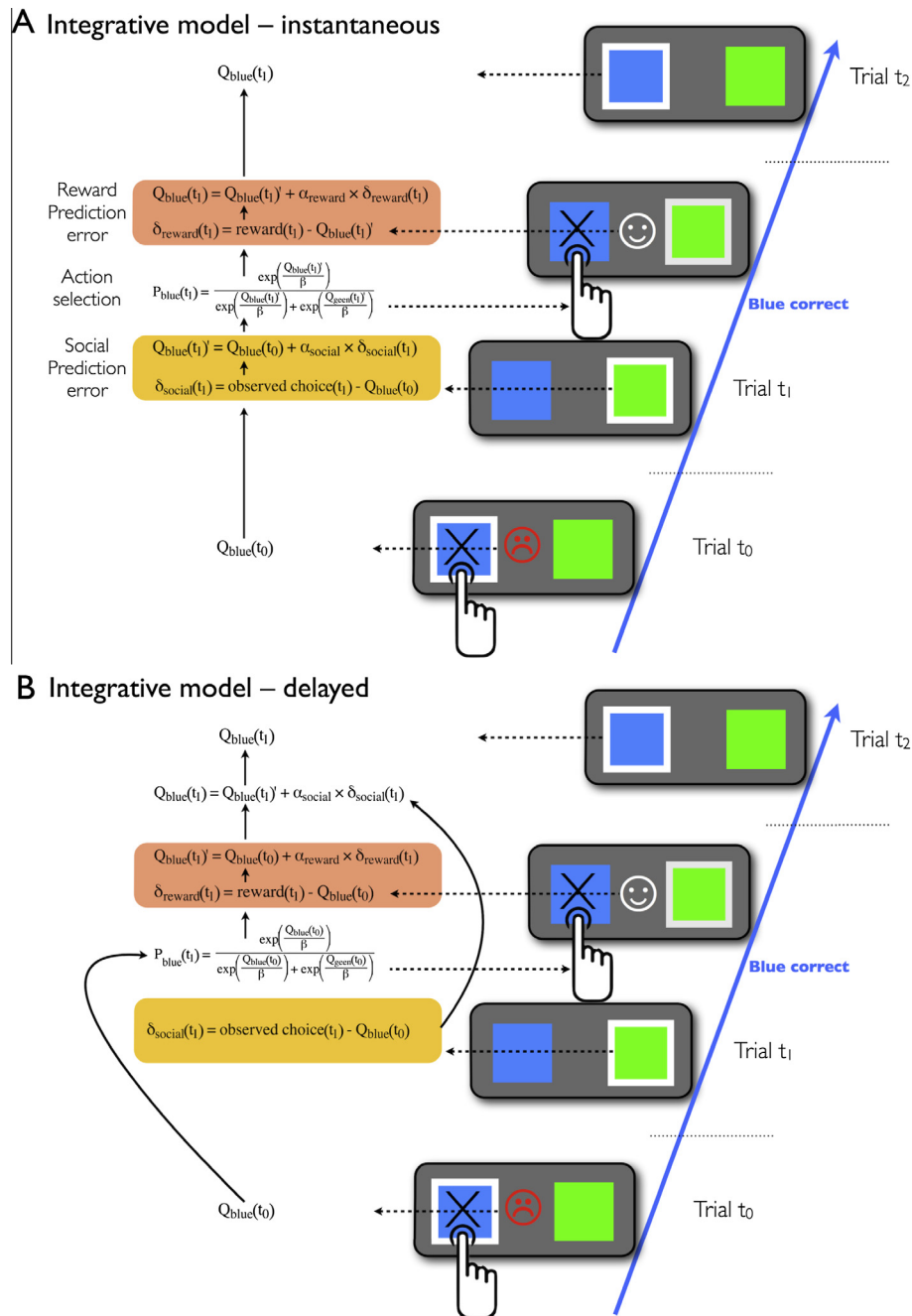
Fig. 2. Schematic illustration of two integrative models used to predict trial-by-trial choices during social reversal learning. (A) Instantaneous integration model. After receiving feedback in trial t_0 , in trial t_1 the participant sees the other player either staying with the previous choice or switching to the other color. The resulting social prediction error \delta_{\text{social}} has a positive (=conservative \delta_{\text{social}} ) or negative (=impulsive \delta_{\text{social}} ) sign and is instantaneously used to update Q_{\text{blue}}(t_0) to Q_{\text{blue}}(t_1) taking into account the social learning rate \alpha_{\text{social}} . Q_{\text{blue}}(t_1) then determines the action selection probability P_{\text{blue}}(t_1) based on a softmax function. After the participant has made his/her choice and the outcome has been received in trial t_1 , Q_{\text{blue}}(t_1) is then updated by the reward prediction error \delta_{\text{reward}} weighted by the reward learning rate \alpha_{\text{reward}} to Q_{\text{blue}}(t_1) . Q_{\text{green}}(t_1) is computed as 1 - Q_{\text{blue}}(t_1) . (B) Delayed integration model. The only difference to the instantaneous integration model is that \delta_{\text{social}} of trial t_1 is not contributing to the action selection probability P_{\text{blue}}(t_1) but becomes only effective after the outcome has been obtained, that is, after Q_{\text{blue}}(t_1) has been updated by \delta_{\text{reward}} to Q_{\text{blue}}(t_1) . (For interpretation of the references to colour in this figure legend, the reader is referred to the web version of this article.)
