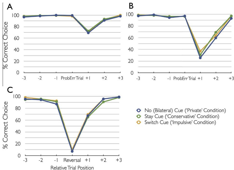
Fig. 6. Choice accuracy as a function of trial position and lateral cue in the non-social control experiment (Study 2). (A, B) Accuracy for trials -3 before to +3 after probabilistic errors (ProbErr), shown for first (A) and late (B) ProbErrs in a reversal episode. (C) Accuracy for trials -3 before to +3 after reversals. Error bars show standard errors of the mean.
