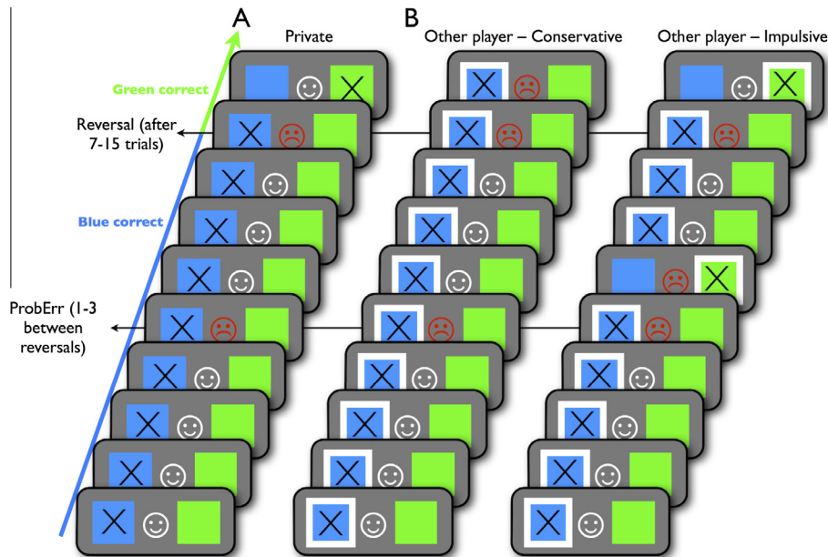
Fig. 1. Design of the social reversal learning task illustrating one reversal episode. (A) Private condition. Crosses illustrate hypothetical choices. Feedback was given instantaneously after a choice had been made. A varying number of probabilistic errors showing ‘wrong’ feedback after correct choices were presented before each reversal. (B) The two social conditions involving the presentation of conservative versus impulsive choices made by a (fictitious) other player who either shared the same birthday as the participant (similar-other group) or not (dissimilar-other group). The other player’s choices were indicated by a white frame surrounding his/her choice before the real participant made his/her choice. Crosses show hypothetical choices reflecting imitative response behavior. Note that participants were exposed to choices made by ONE other player who displayed conservative AND impulsive choices in different reversal episodes. As illustrated, the number of errors made by the other player was balanced between the conservative and impulsive condition.
